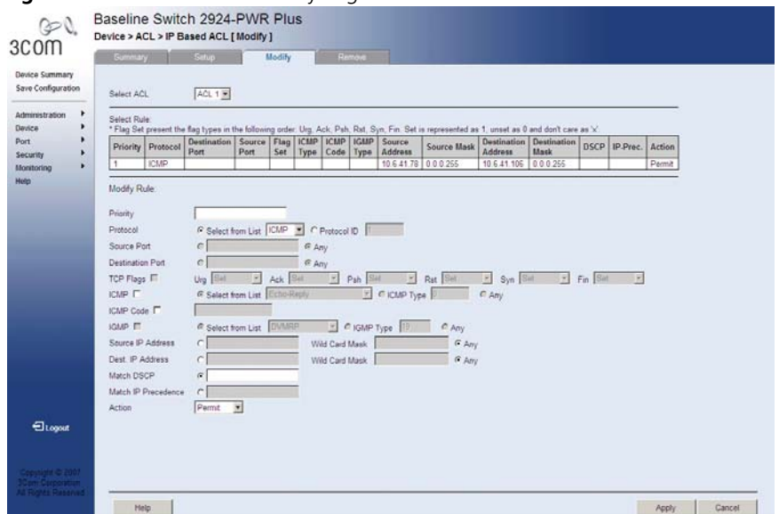
Figure 33 IP Based ACL Modify Page
