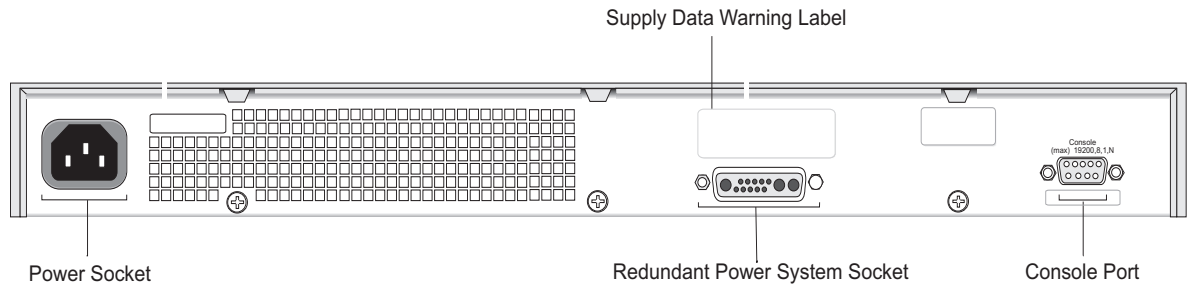
Switch 4200 Series — Rear View Detail Figure 4 Switch 4200 Series — rear view
