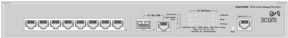
Figure 1 OfficeConnect Managed Fast Ethernet PoE Switch—front panel.
