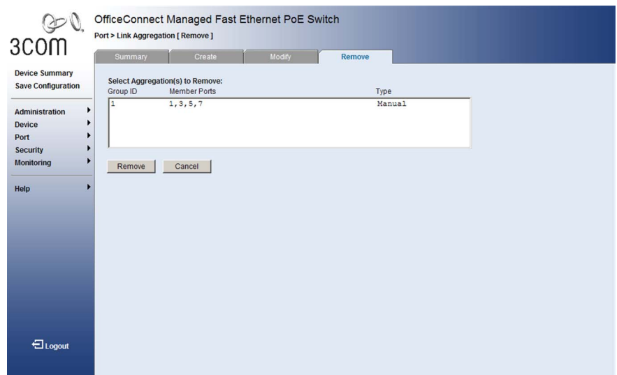
Figure 64 Link Aggregation Remove Page
