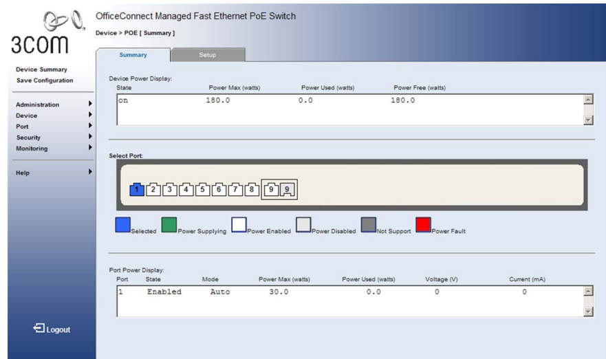
Figure 106 Port PoE Summary Page
