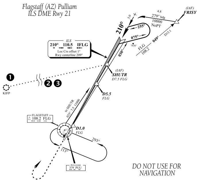
Figure 6-62 ILS Approach, Flagstaff
