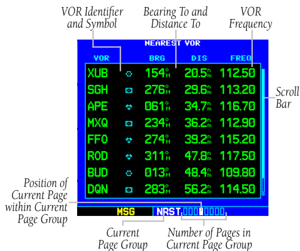
Figure 8-13 Nearest VOR Page
