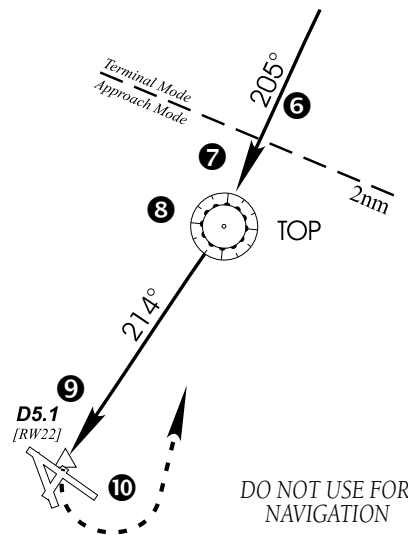
Figure 6-46 Approach Mode
