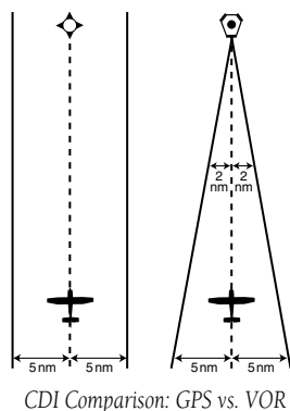
Figure C-8 CDI Comparison
