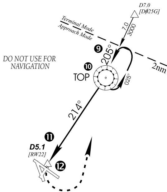
Figure 6-38 Approach Mode
