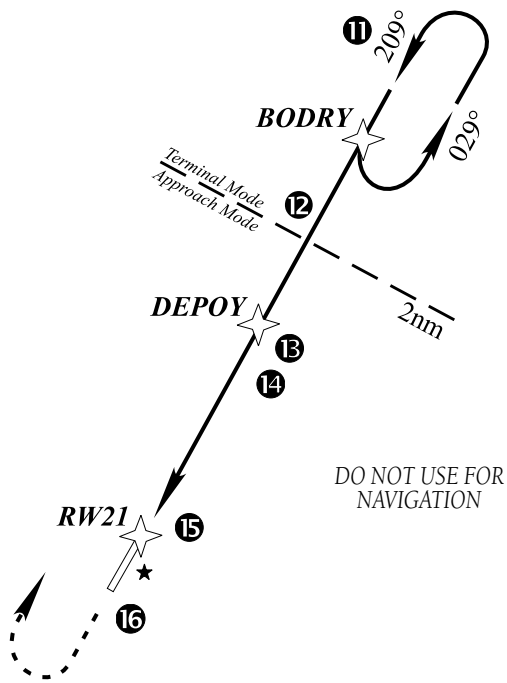
Figure 6-29 Approach Mode
