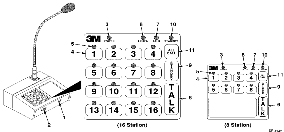
Figure 3. Station Selector, Controls, and Indicators
