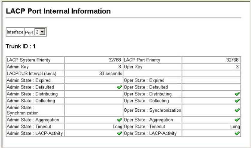
Figure 3-58 LACP - Port Internal Information
