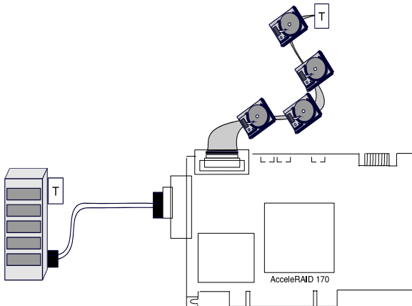
Figure 2-8. Connecting Disk Drives to the AcceleRAID 170
