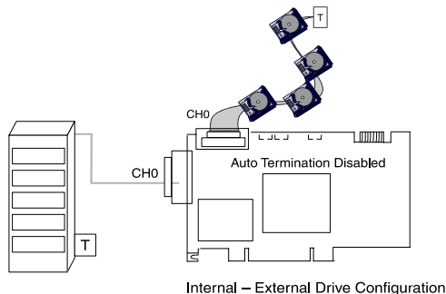
Figure 2-11. Termination with Internal and External Drive Configuration
