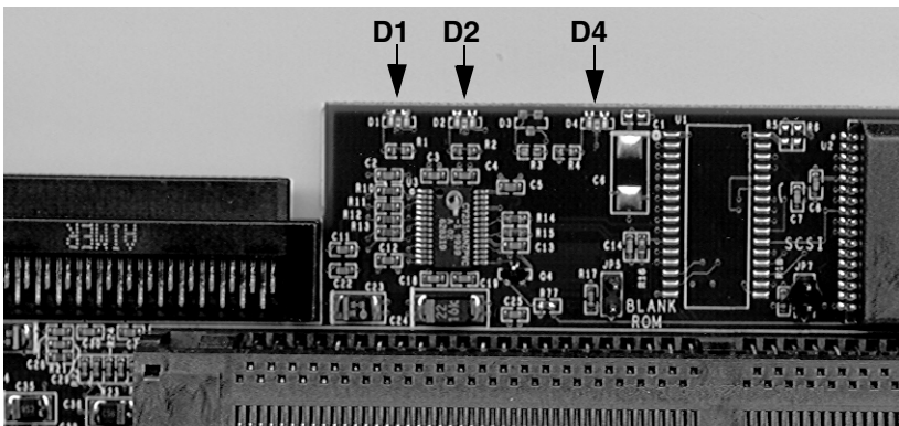
Figure 2-2. AcceleRAID 170 LEDs
