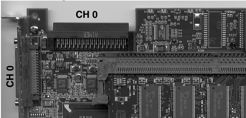
Figure 2-1. AcceleRAID 170 Controller Channel Connectors
