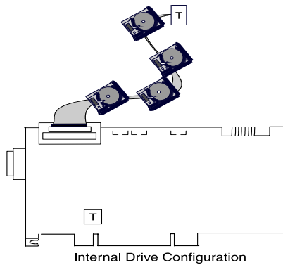
Figure 2-9. Termination with Internal Drive Configuration
