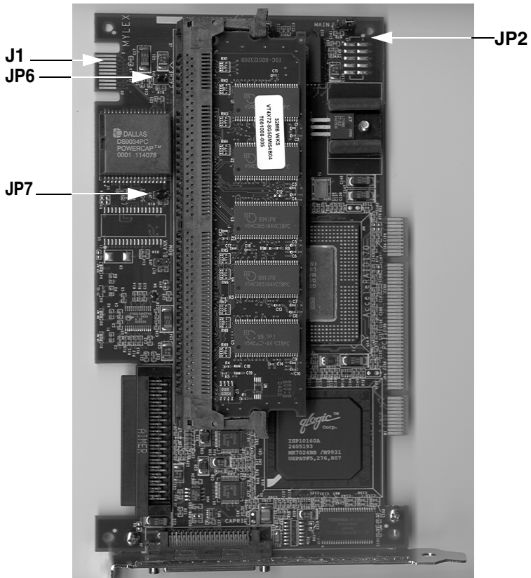
Figure 2-3. AcceleRAID 170 Jumper Locations
