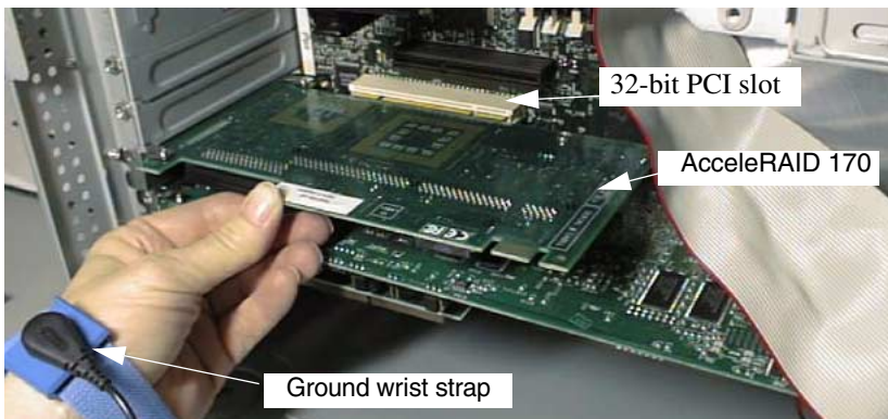
Figure 2-7. Plug the Controller into any 32-bit or 64-bit PCI Slot
