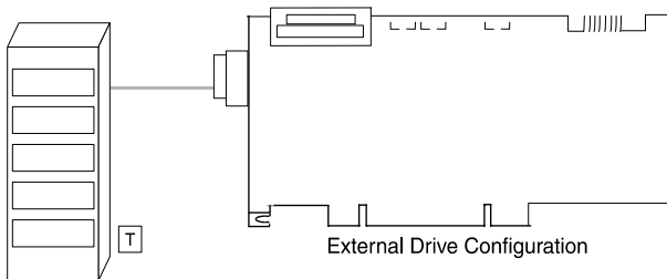
Figure 2-10. Termination with External Drive Configuration
