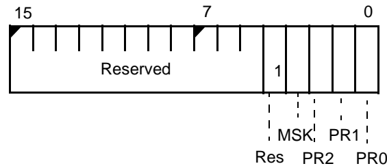
Figure 8-9 Serial Port Interrupt Control Register (SPICON, offset 44h)
