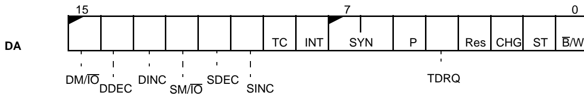
DMA 1 Control Register (D1CON) Page 10-3
