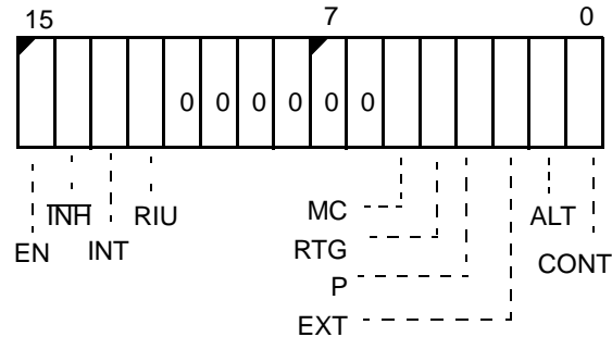
Figure 9-1 Timer 0 and Timer 1 Mode and Control Registers (T0CON, T1CON, offsets 56h and 5Eh)
