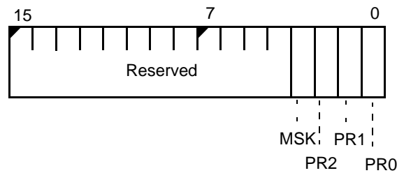
Figure 8-19 Timer and DMA Interrupt Control Registers (T0INTCON, T1INTCON, T2INTCON, DMA0CON, DMA1CON, offsets 32h, 38h, 3Ah, 34h, and 36h)
