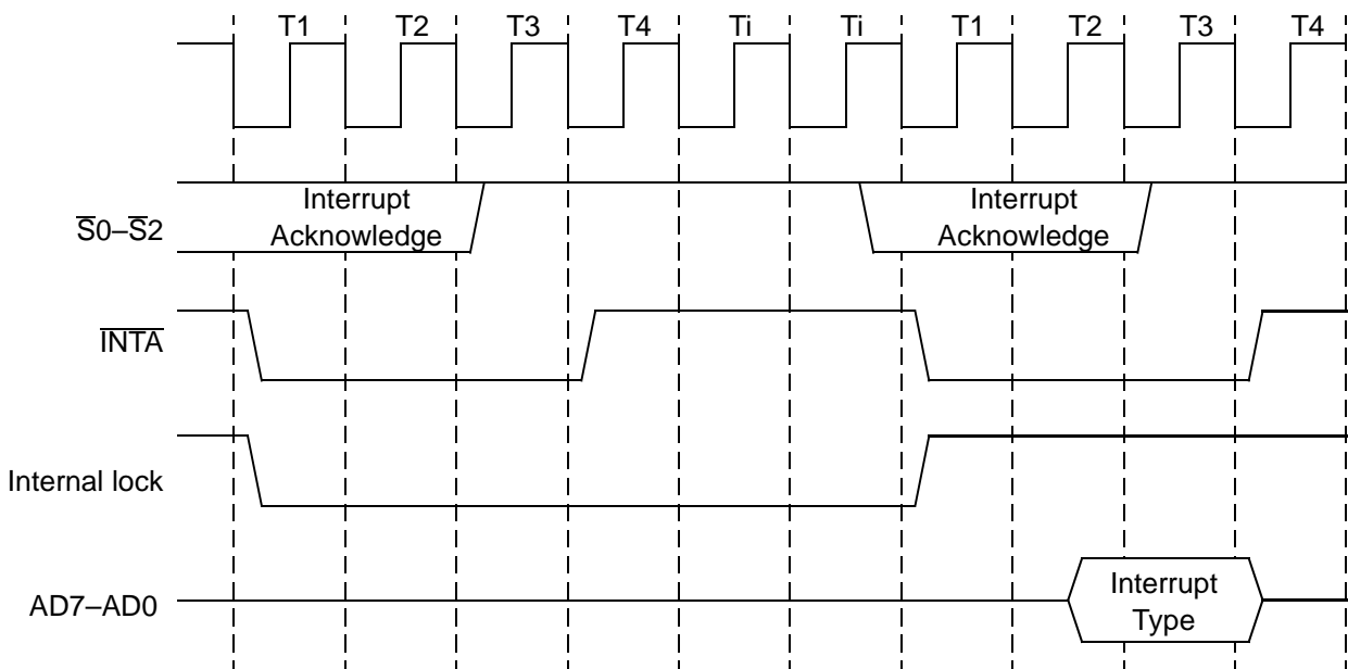
Figure 8-1 External Interrupt Acknowledge Bus Cycles
