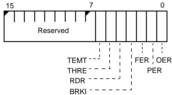
Figure 11-2 Serial Port Status Register (SPSTS, offset 82h)
