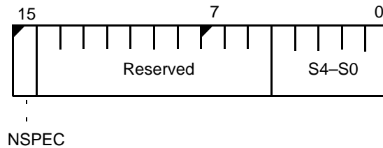
Figure 8-18 End-of-Interrupt Register (EOI, offset 22h)
