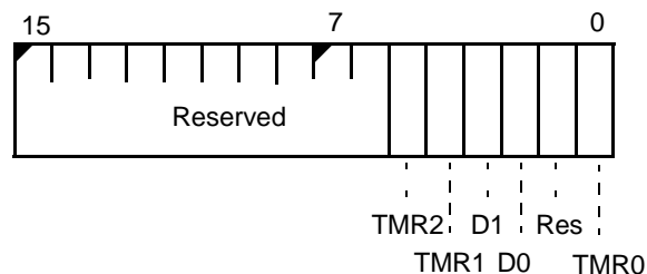
Figure 8-24 Interrupt Mask Register (IMASK, offset 28h)
