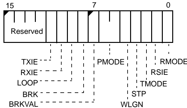
Figure 11-1 Serial Port Control Register (SPCT, offset 80h)
