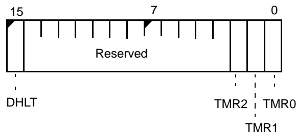
Figure 8-10 Interrupt Status Register (INTSTS, offset 30h)
