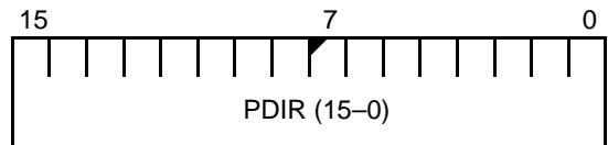
Figure 13-5 PIO Direction 0 Register (PDIR0, offset 72h)
