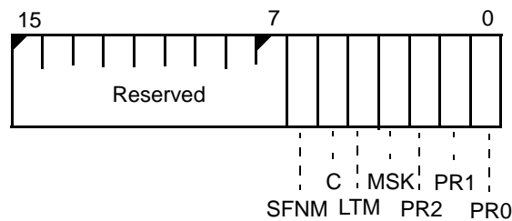
Figure 8-4 INT0 and INT1 Control Registers (IOCON, I1CON, offsets 38h and 3Ah)
