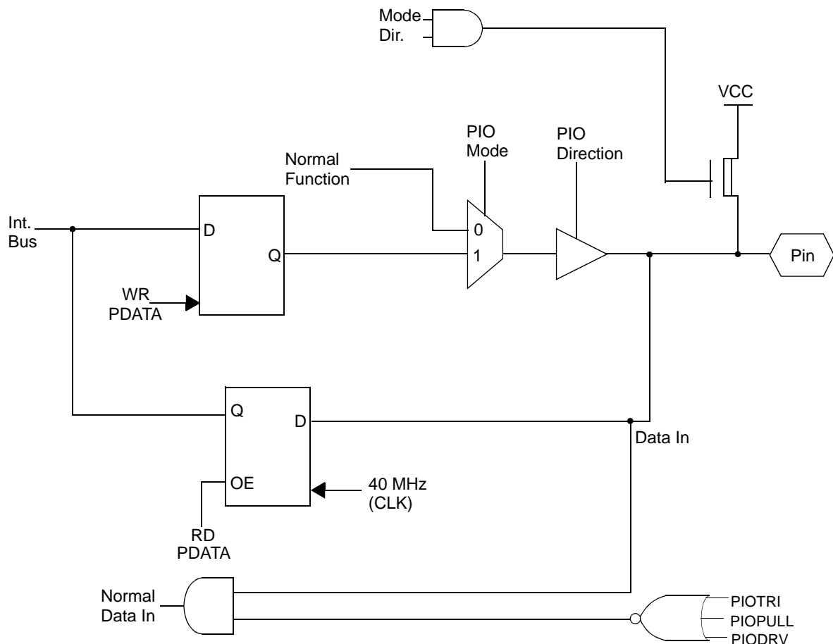
Figure 13-1 Programmable I/O Pin Operation
