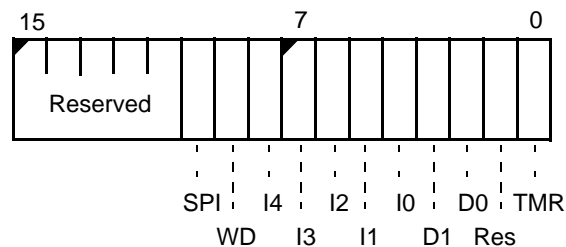
Figure 8-14 Interrupt Mask Register (IMASK, offset 28h)
