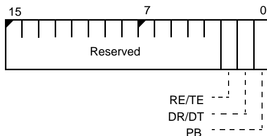
Figure 12-1 Synchronous Serial Status Register (SSS, offset 10h)
