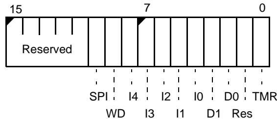
Figure 8-11 Interrupt Request Register (REQST, offset 2Eh)
