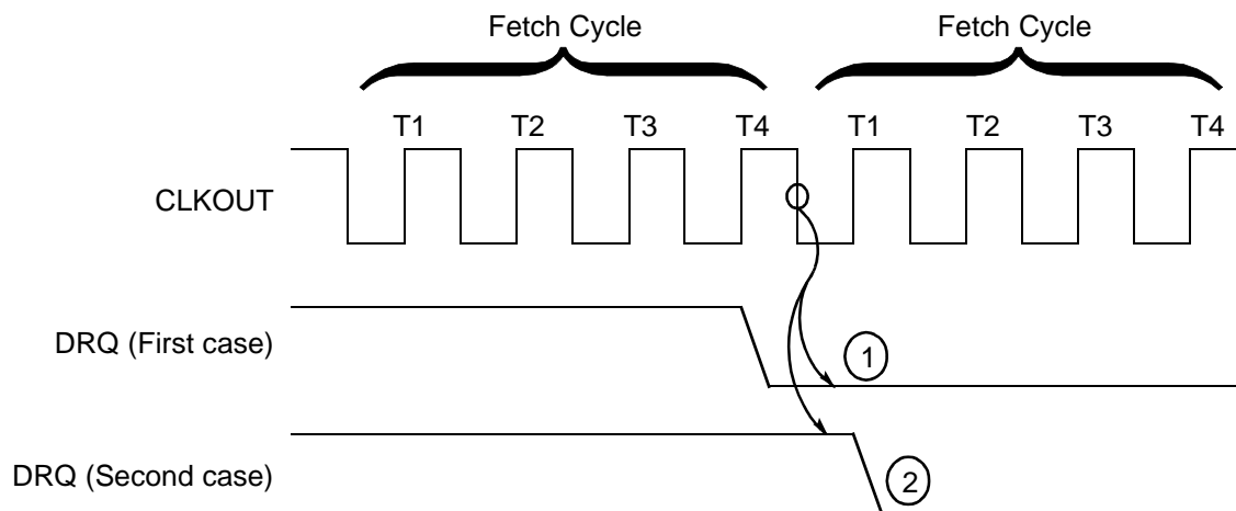
Figure 10-8 Source-Synchronized DMA Transfers
