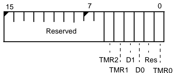
Figure 8-22 In-Service Register (INSERTV, offset 2Ch)
