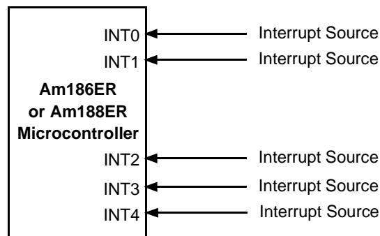
Figure 8-2 Fully Nested (Direct) Mode Interrupt Controller Connections
