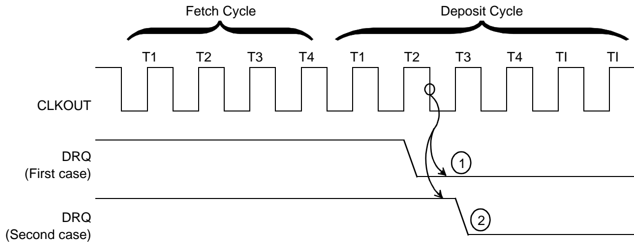
Figure 10-9 Destination Synchronized DMA Transfers
