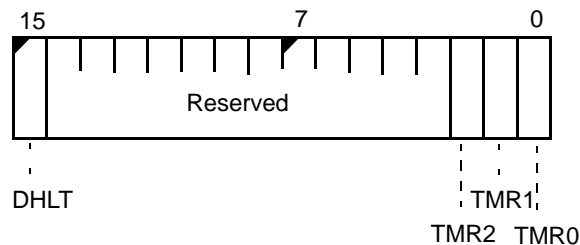
Figure 8-20 Interrupt Status Register (INTSTS, offset 30h)
