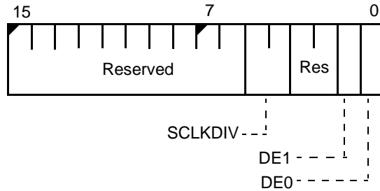
Figure 12-2 Synchronous Serial Control Register (SSC, offset 12h)
