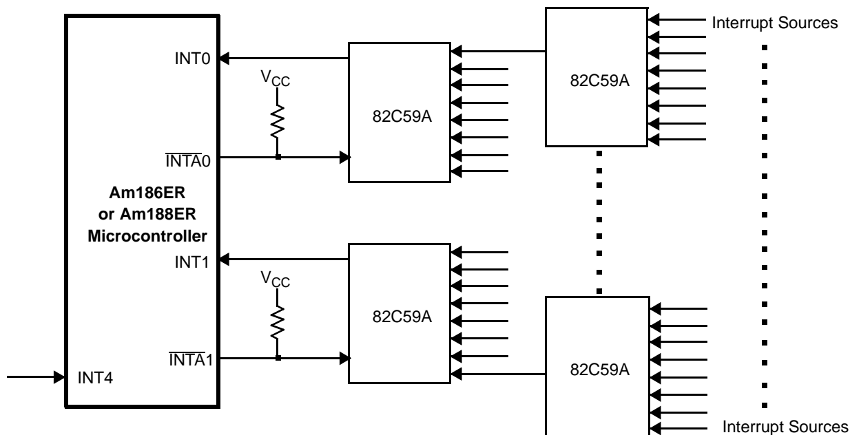
Figure 8-3 Cascade Mode Interrupt Controller Connections
