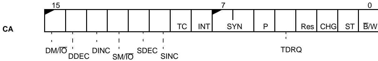
Figure A-1 Internal Register Summary (continued)
