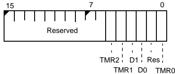
Figure 8-21 Interrupt Request Register (REQST, offset 2Eh)
