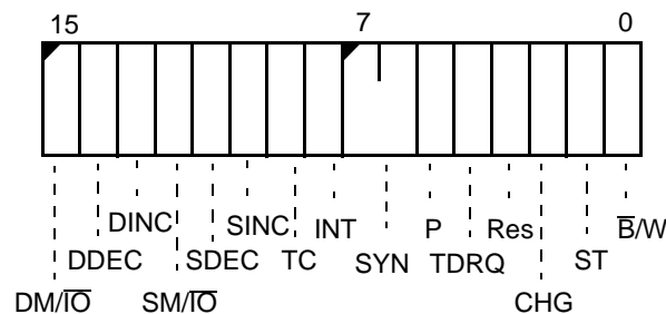
Figure 10-2 DMA Control Registers (D0CON, D1CON, offsets CAh and DAh)
