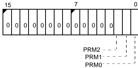
Figure 8-13 Priority Mask Register (PRIMSK, offset 2Ah)
