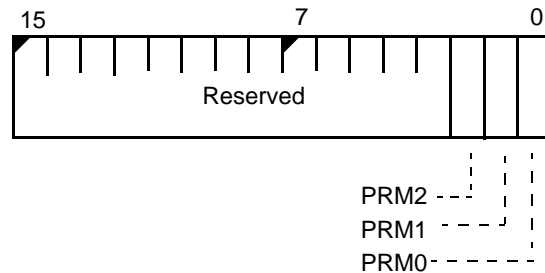
Figure 8-23 Priority Mask Register (PRIMSK, offset 2Ah)
