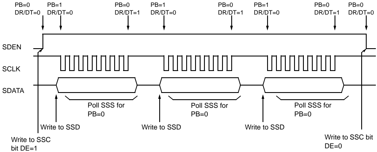
Figure 12-5 Synchronous Serial Interface Multiple Write
