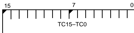
Figure 9-4 Timer Maxcount Compare Registers (TOCMPA, TOCMPB, T1CMPA, T1CMPB, T2CMPA, offsets 52h, 54h, 5Ah, 5Ch, and 62h)
