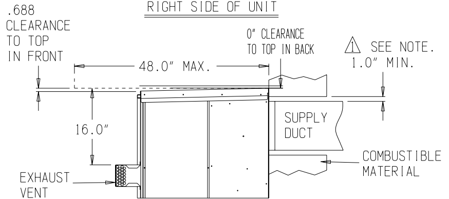
FIGURE 1 COMBUSTIBLE CLEARANCE
