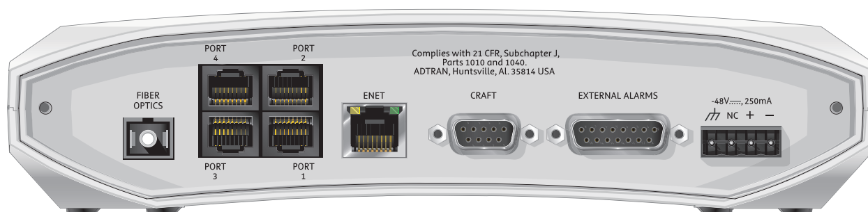
Figure 3. NTU-8F Rear Panel Connections
