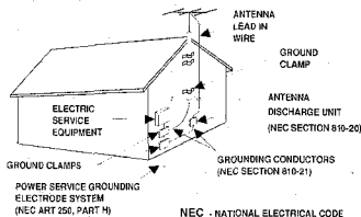
EXAMPLE OF ANTENNA GROUNDING ACCORDING TO NATIONAL ELECTRICAL CODE, ANSI/NFPA 70
