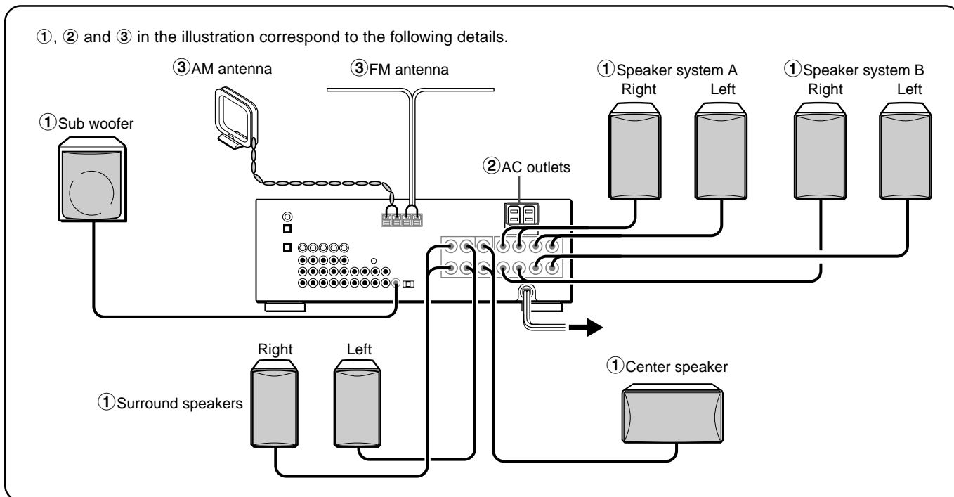
Front speakers
