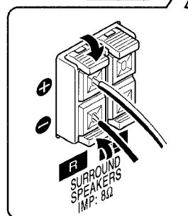
Surround speakers
