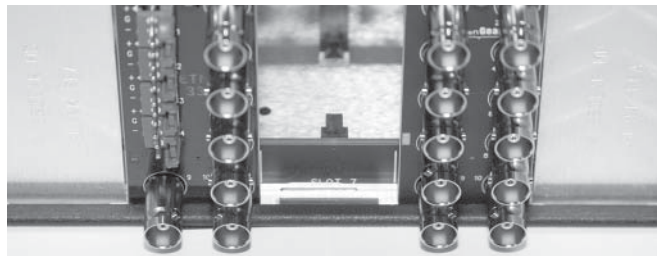
openGear frame with a modular rear panel
