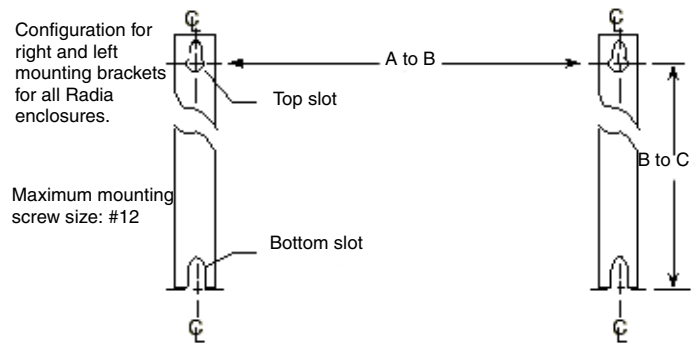
FIG. 2 Bracket configuration
