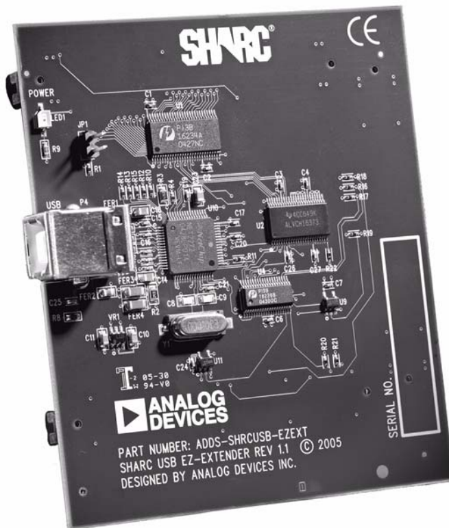
Figure 2-14. SHARC USB EZ-Extender
