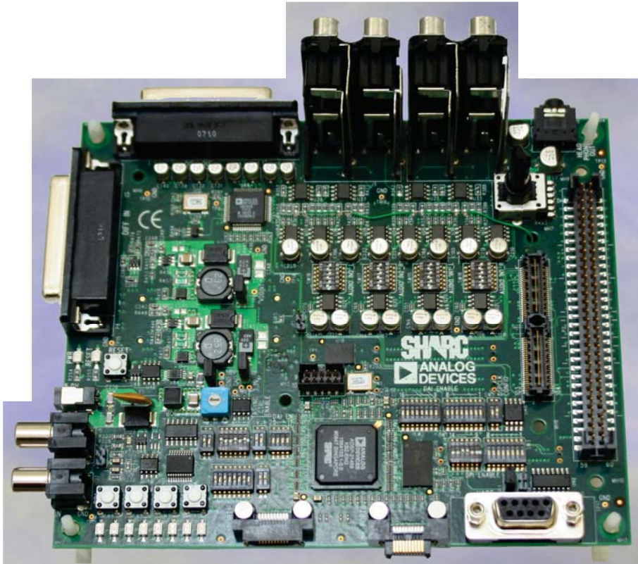
Figure 2-4. ADSP-21469 EZ-KIT Lite Evaluation System
