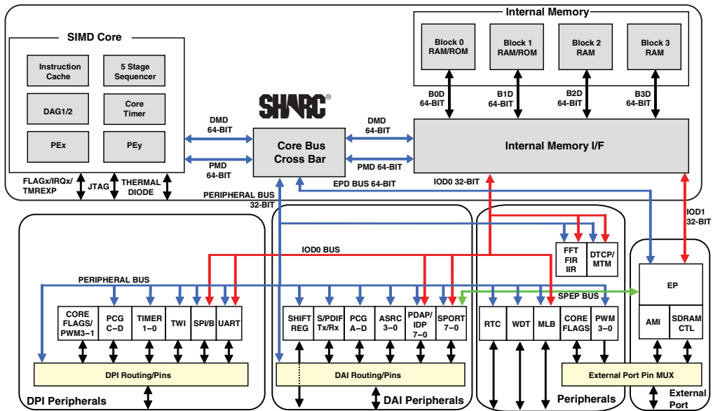
Figure 1-1. ADSP-2147x Processor Block Diagram
