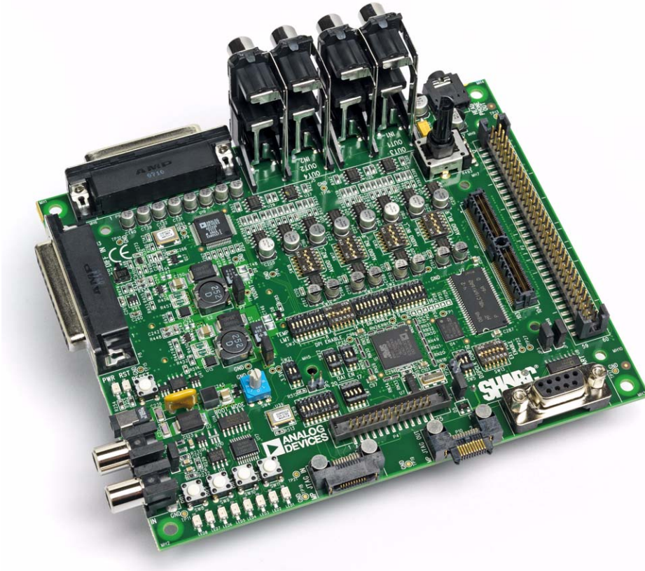
Figure 2-11. ADSP-21479 EZ-Board
