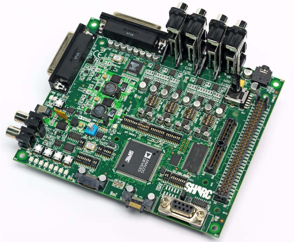
Figure 2-10. ADSP-21489 EZ-Board
