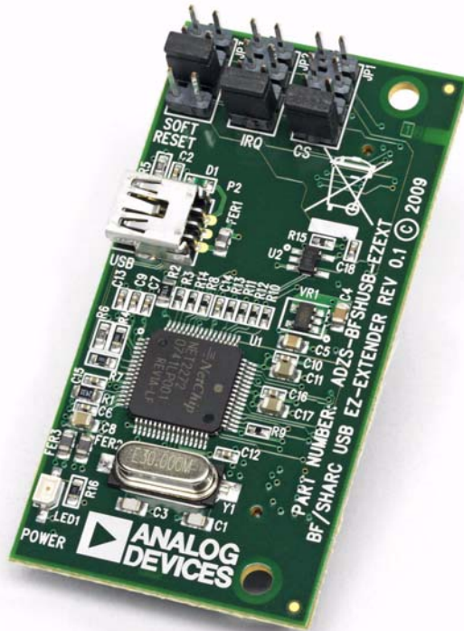
Figure 2-17. Blackfin/SHARC USB EZ-Extender
