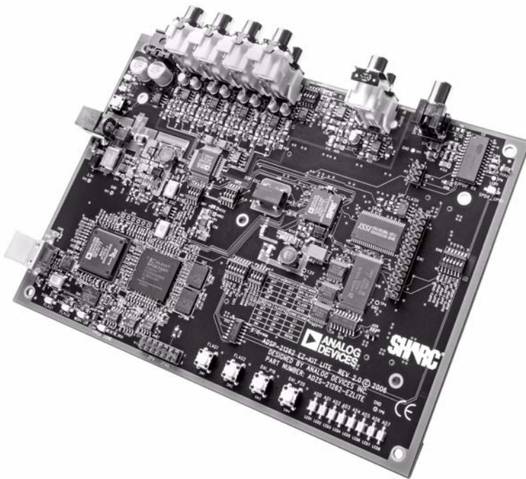
Figure 2-9. ADSP-21262 EZ-KIT Lite Evaluation System
