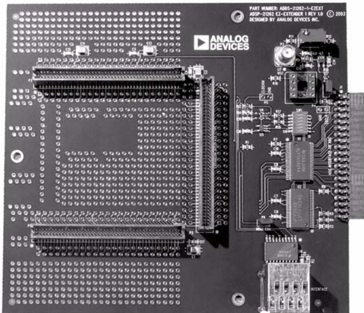
Figure 2-15. SHARC EZ-Extender
