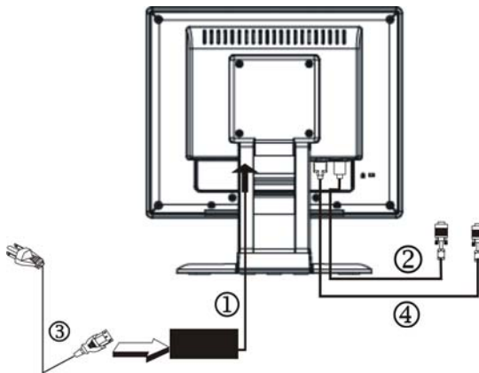
Figure 1 Connecting Cables
