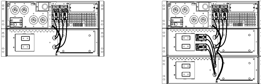
Battery Connections
