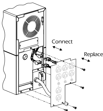
Figure 1: Tower UPS and plate configuration
