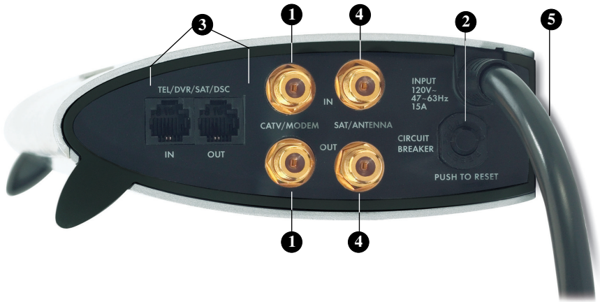
Figure 4. C5 Side Panel Connectors
