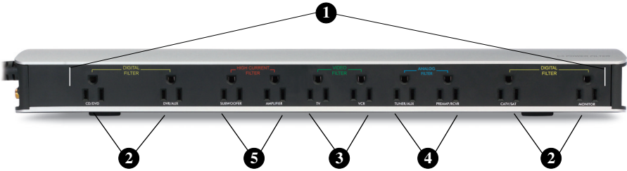
Figure 3. C5 Outlet Panel
