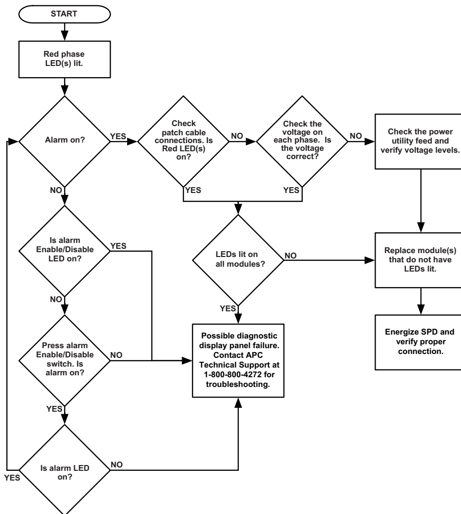
Figure 9: Troubleshooting Flowchart
