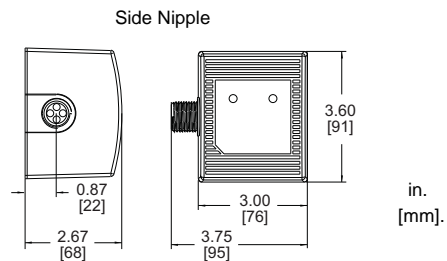
Figure 4: Dimensions
