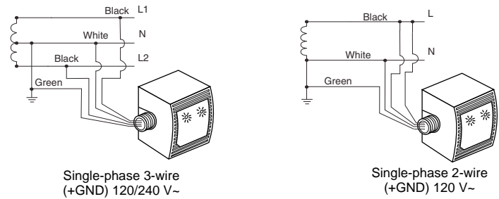
Figure 2: Wiring
