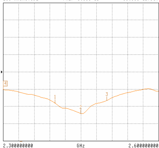
S11 FORWARD REFLECTION
