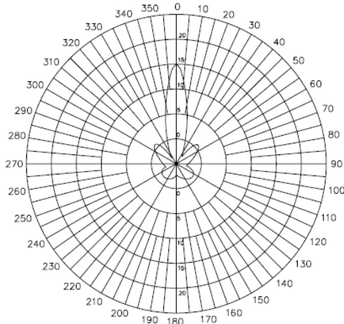
E-Plane Field Patterns for 5.8GHz
