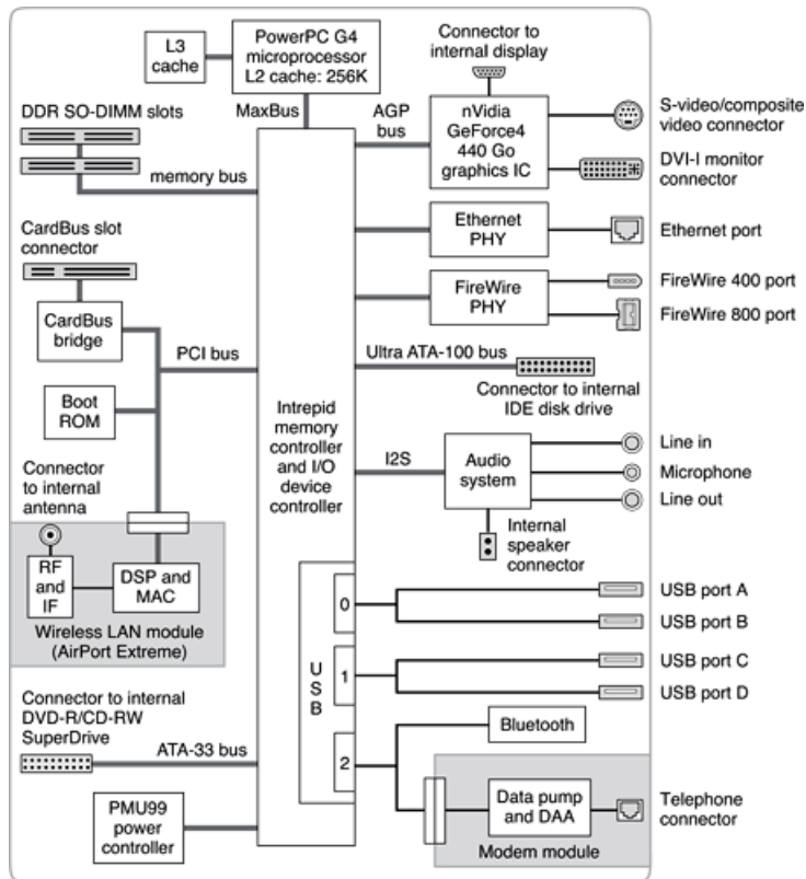
Figure 2-1 Block diagram
