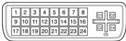
Figure 3-9 DVI-I connector
