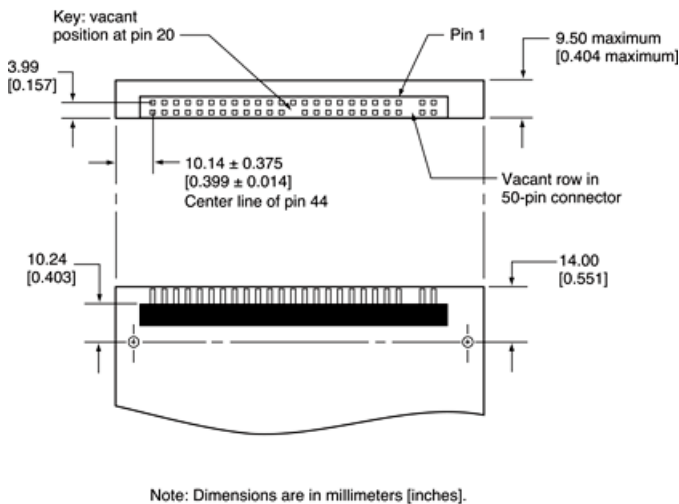
Figure 3-5 Hard disk connector and location
