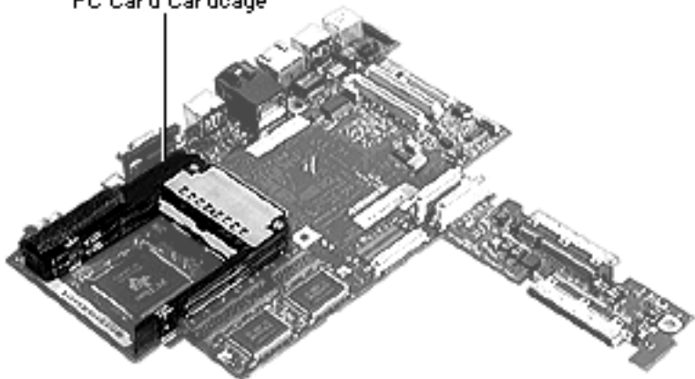
PC Card Cardcage
