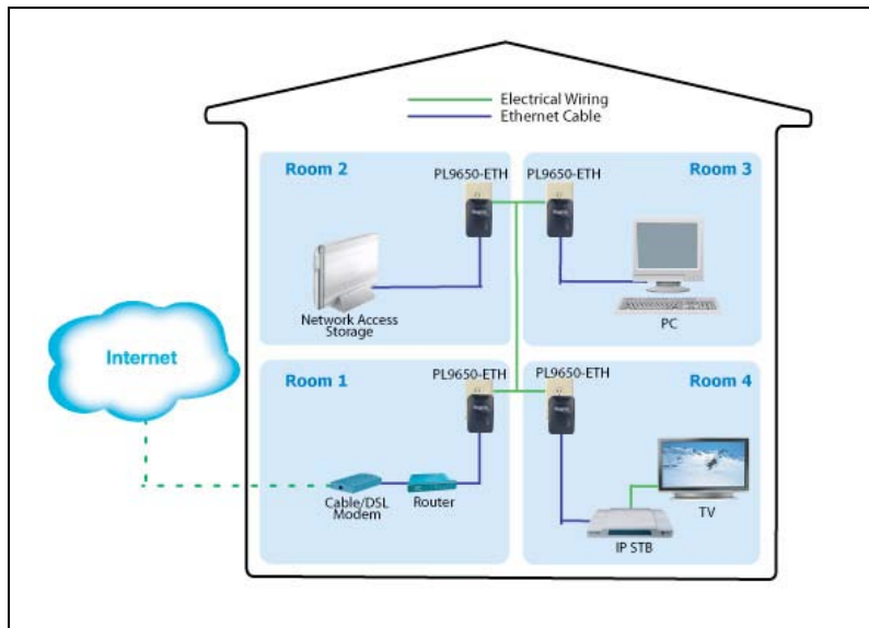
Figure: 4-3: Networking other Ethernet enabled devices.
