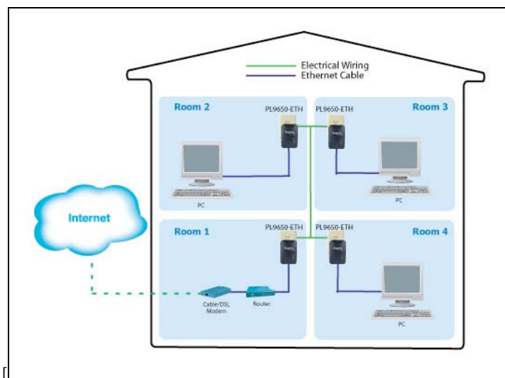
Figure 4-2: Sharing broadband connection network diagram.
