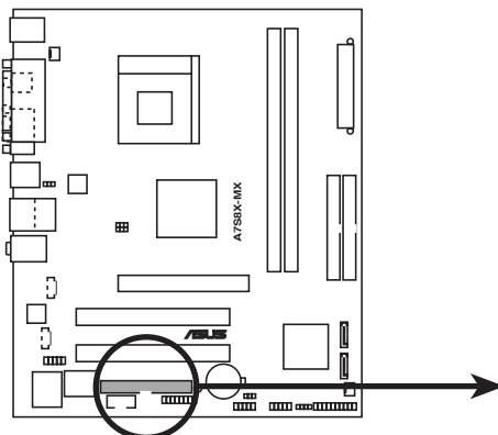
A7S8X-MX Floppy disk drive connector
