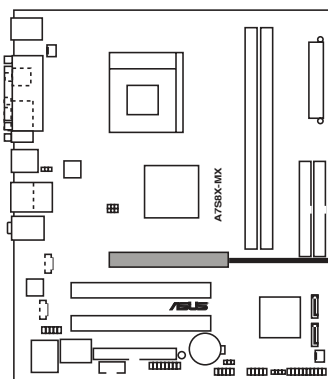
A7S8X-MX Accelerated Graphics Port (AGP1)
