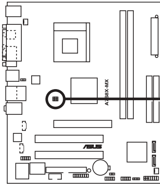
A7S8X-MX External frequency selection
