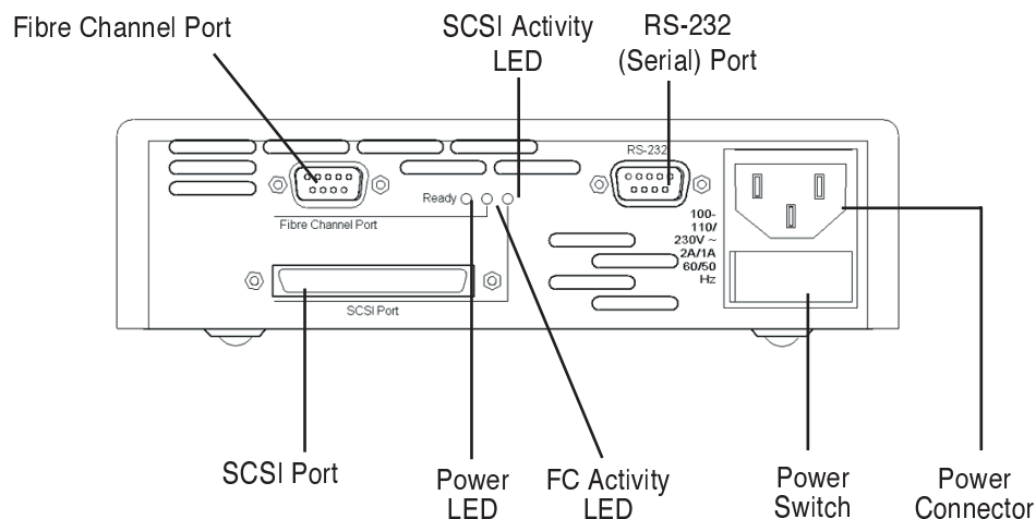
Figure 1: Rear Panel
