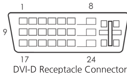
Digital-Only Connector Pin Assignments
