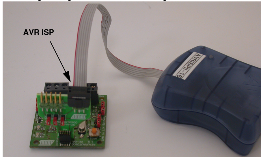
Figure 2-8. Programming the ATAVRAUTO100 using ATAVRAUTO900
