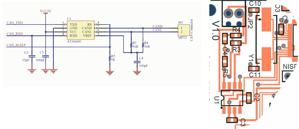
Figure 2-5. CAN High Speed connections
