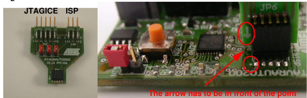
Figure 2-7. ATAVRAUTO900 Connection
