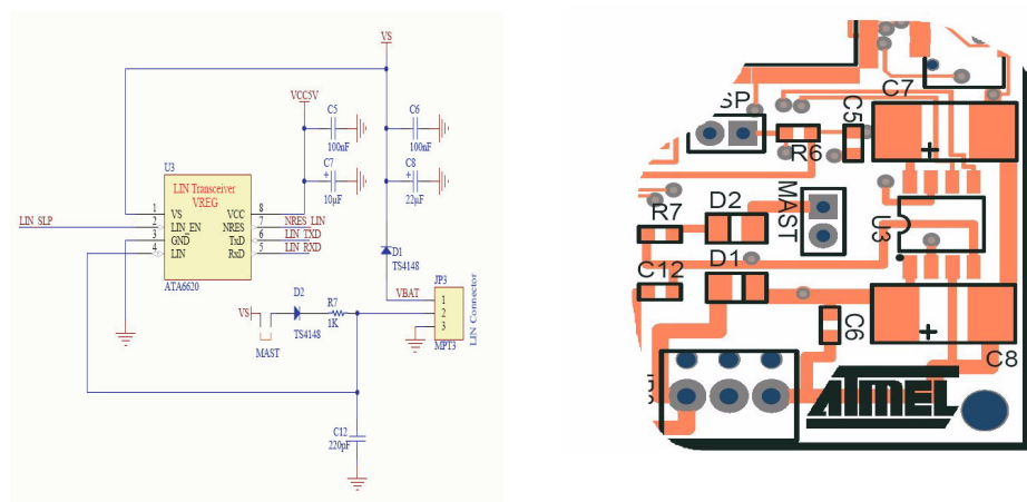
Figure 2-4. .LIN And Power-supply Connections to JP3
