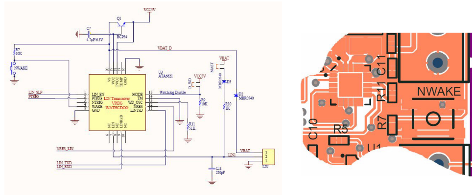
Figure 2-2. The LIN power line is used to bias the ATAVRAUTO100
