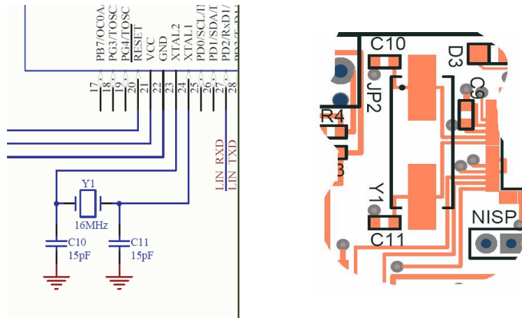
Figure 2-3. Crystal Oscillator connection.
