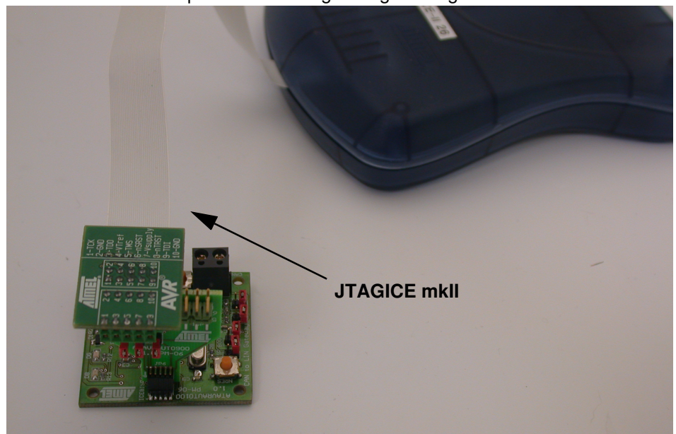
Figure 2-9. JTAGICEmkII probe connecting through debugWIRE interface.
