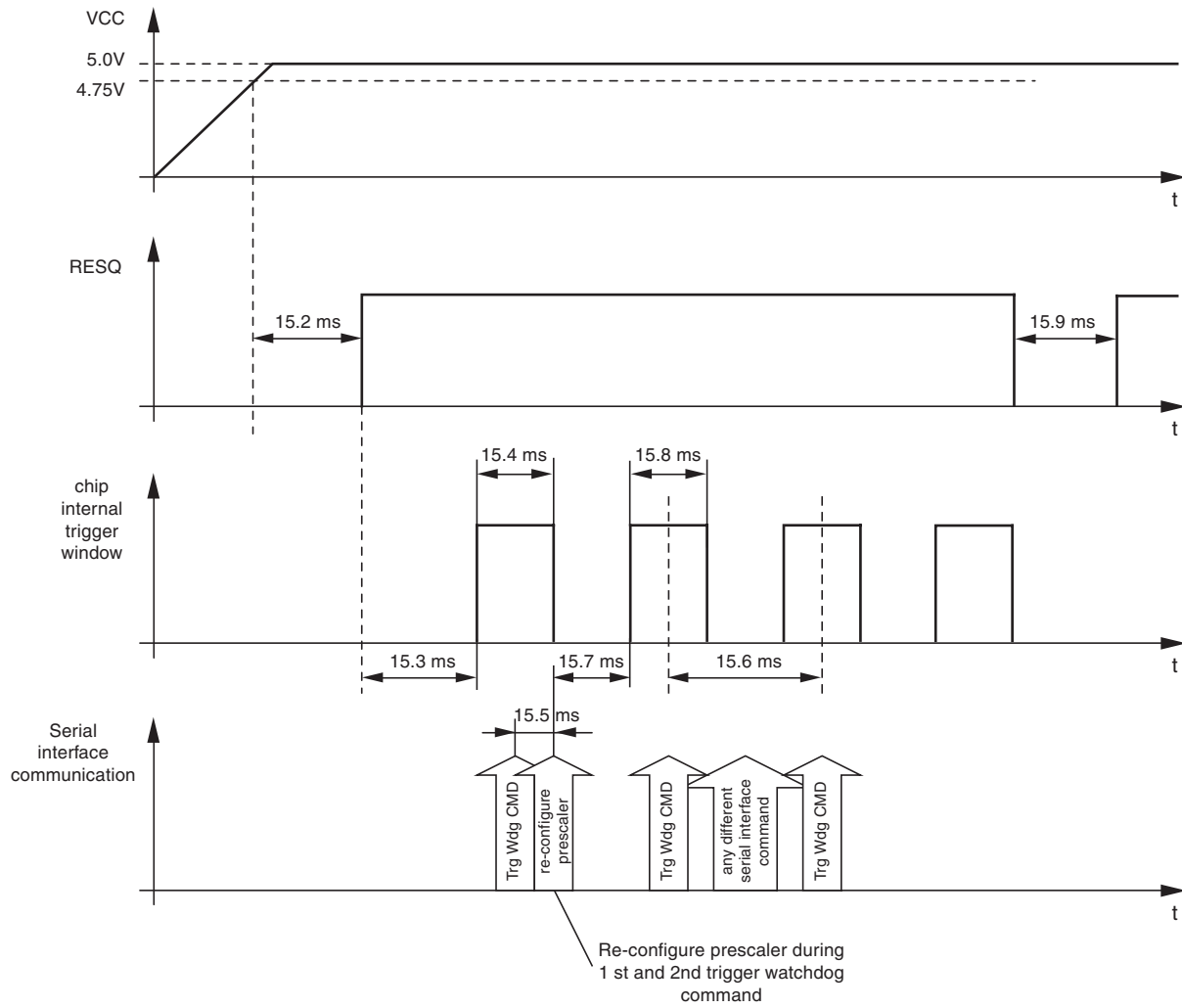
Figure 16-5. Watchdog Trigger
