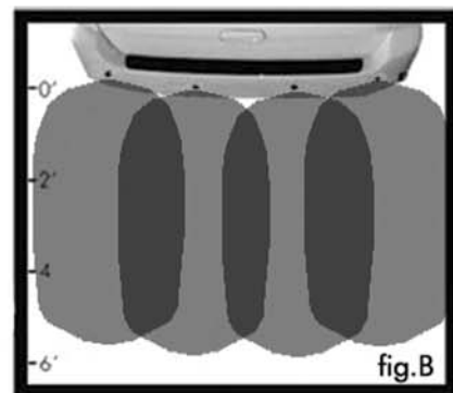
Optional 4 sensor configuration. Approximately 6' of central coverage and selectable outer coverage ranges of 3' (fig.A) or 6' (fig.B). Center sensors use CL & CR ports and outer sensors use L & R ports. (fig.A is a passenger vehicle option and fig.B is a commercial option)
