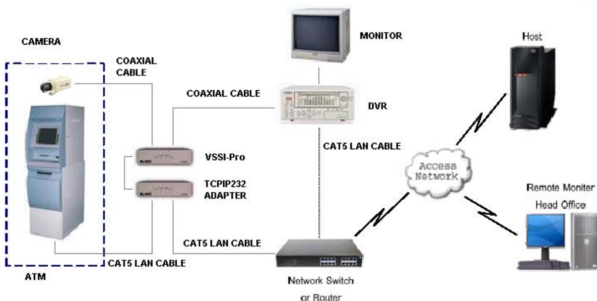
Figure 2. VSSI-Pro Interface
