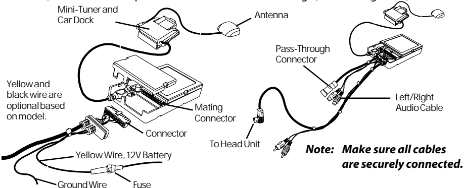
Download from www.researchanddownload.com Figure 1 PIA Cable Interface
