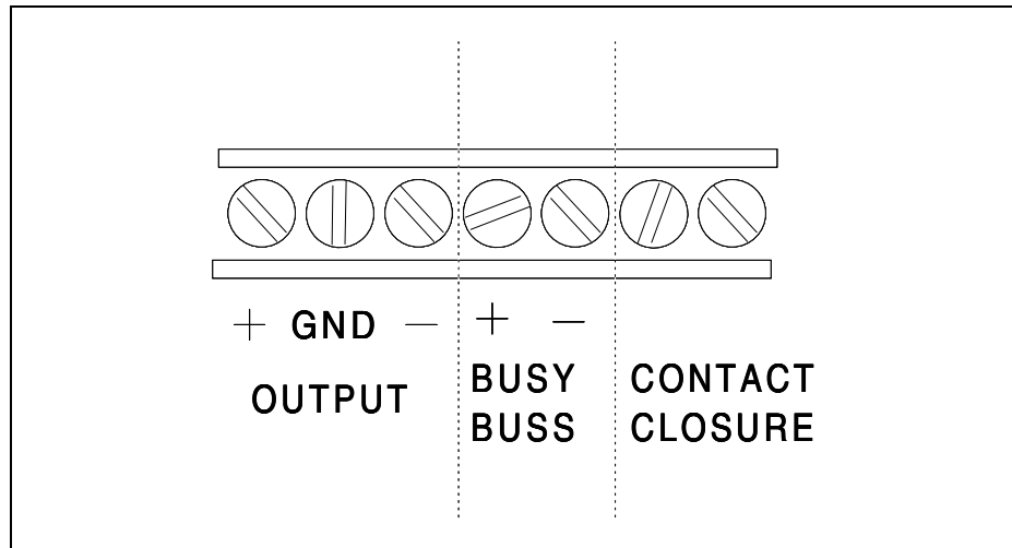
Figure 3. Wiring Connections on Microphone Terminal Block
