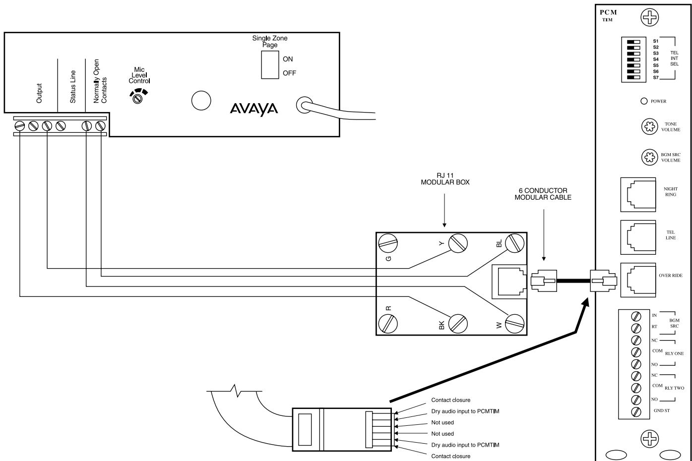
Figure 5. Typical Connections to a LUPCM Paging System Controller Unit
