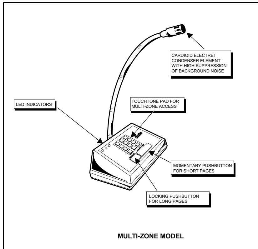
Figure 1. Multi-Zone Microphone Features
