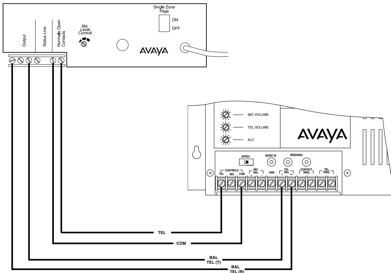
Figure 4. Typical Connections to a Telephone Paging Amplifier
