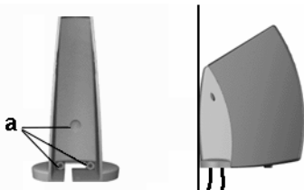
Figure 4-1 Punch Screw Holes and Mount the Residential Gateway-I to a Wall
