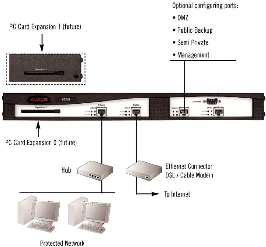
Figure 1 Typical SG203/SG208 security gateway installation
