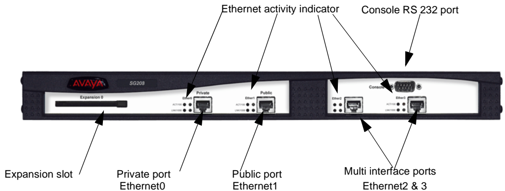
Figure 3 Back panel
