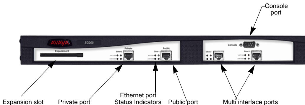
Figure 5 Front panel of the security gateway
