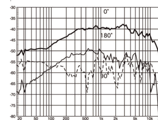
Frequency Response
