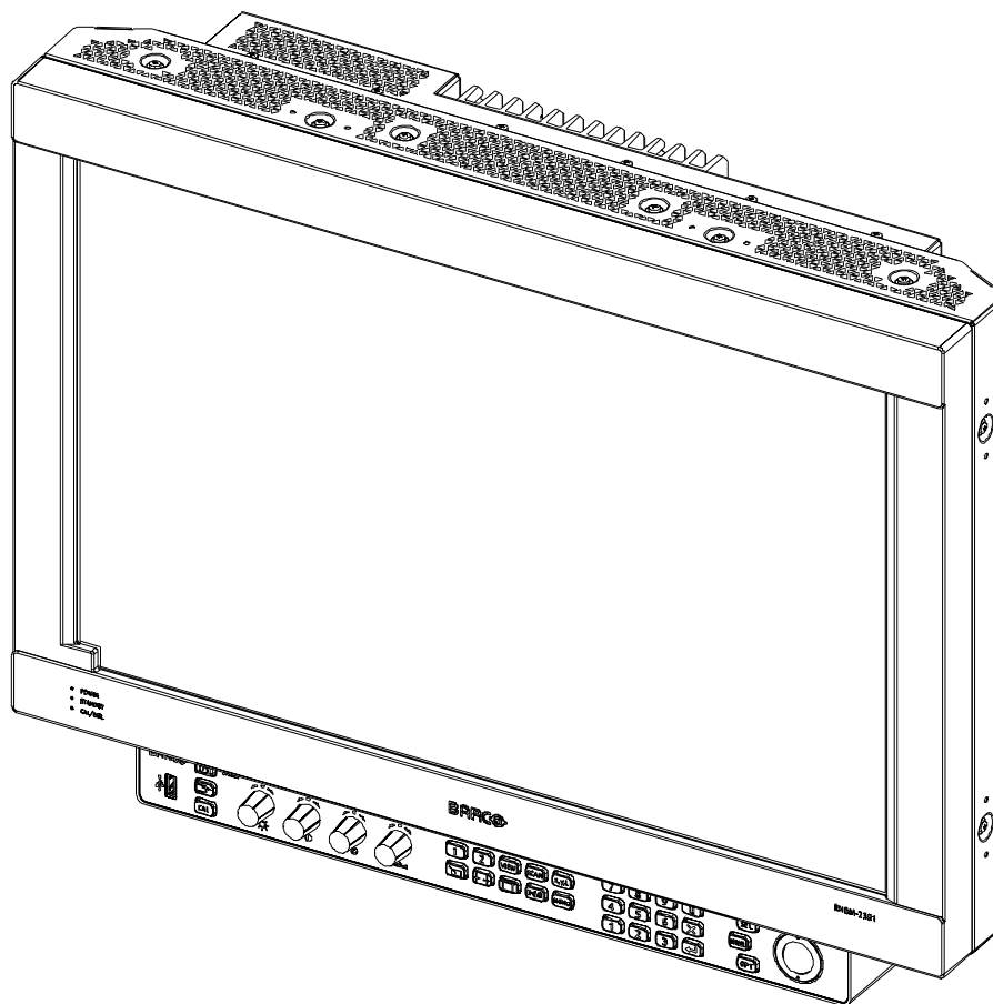
Figure 66: RHDM-2301 Auxiliary view (front)
