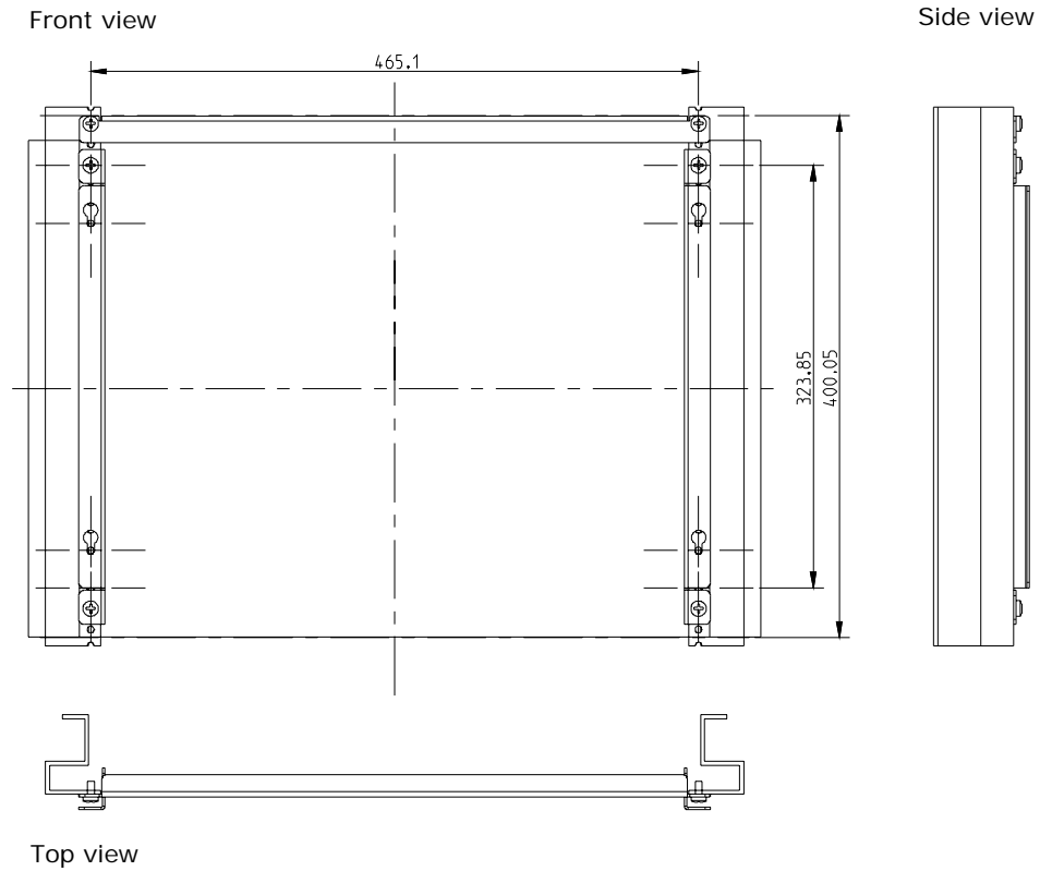
Figure 77: Front, top and side view of the mounted rack and cover brackets
