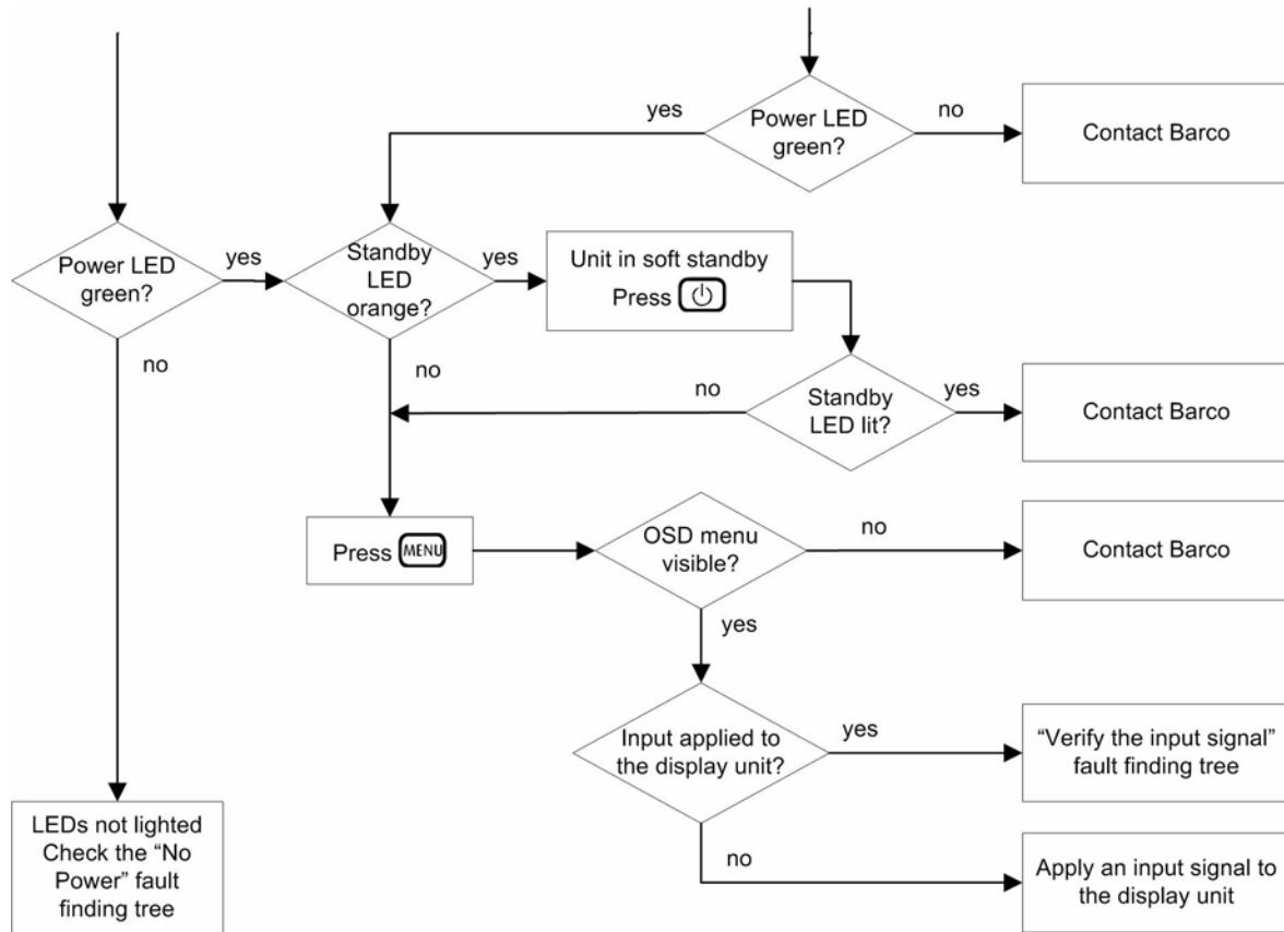
Figure 82: "Nothing observed on the screen" fault finding tree
