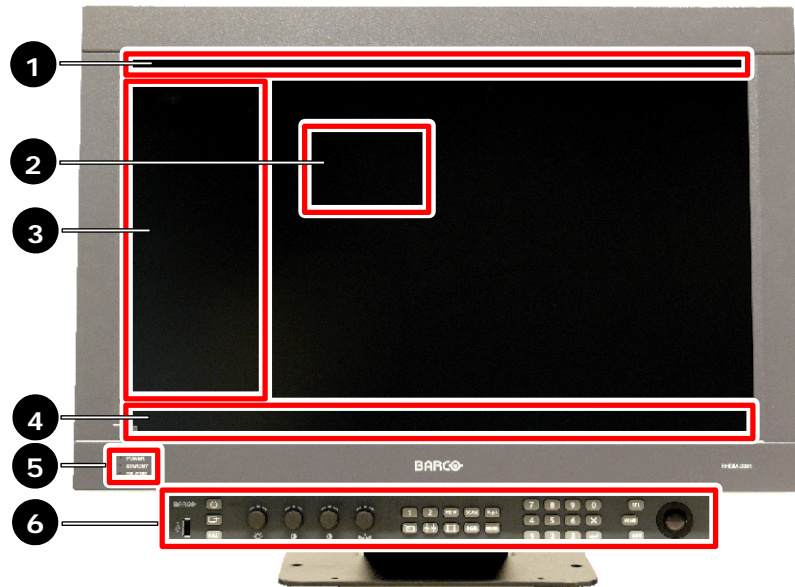
Figure 20: Overview of operational controls, indicators and OSD functionalities
