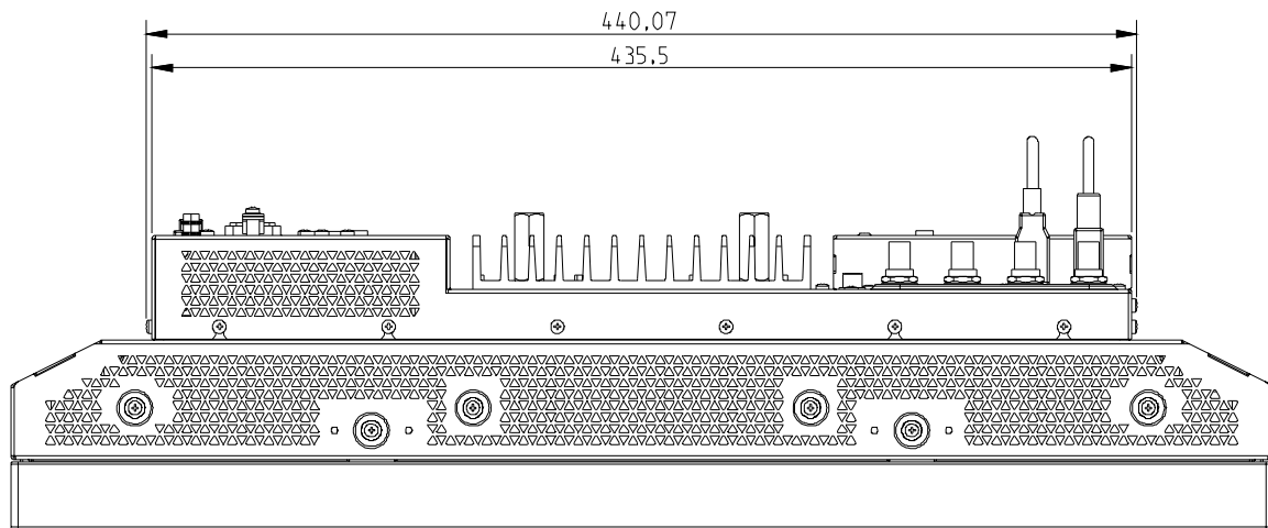
Figure 63: RHDM-2301 Top view (metric units (mm))
