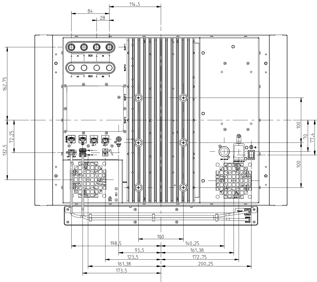
Figure 64: RHDM-2301 Rear view (metric units (mm))
