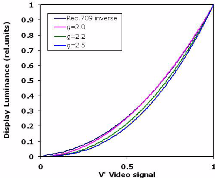
Figure 56: The inverse of the Rec.709 encoding function fitted with a power function
