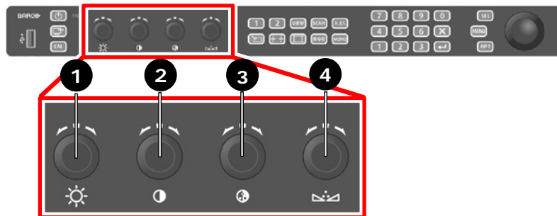
Figure 7: Location of the image adjustment rotary knobs on the control panel
