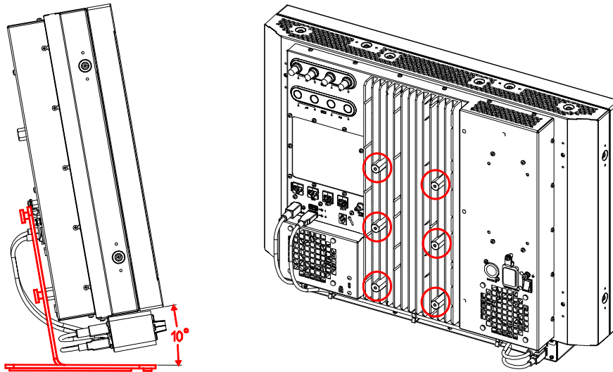
Figure 69: Display unit mounted on Barco stand – VESA mount positions
