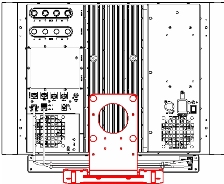
Figure 71: Mounting of the Barco stand – rear view
