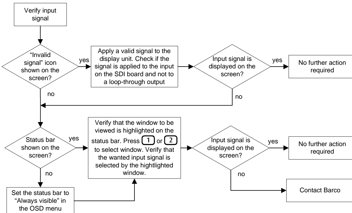
Figure 83: "Verify input signal" fault finding tree
