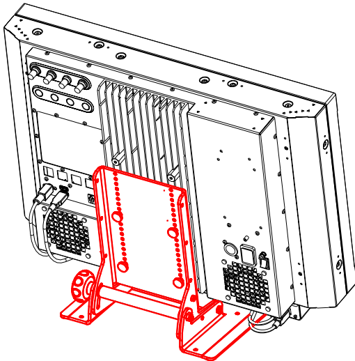
Figure 73: Rear side of the display unit with mounted tiltable stand
