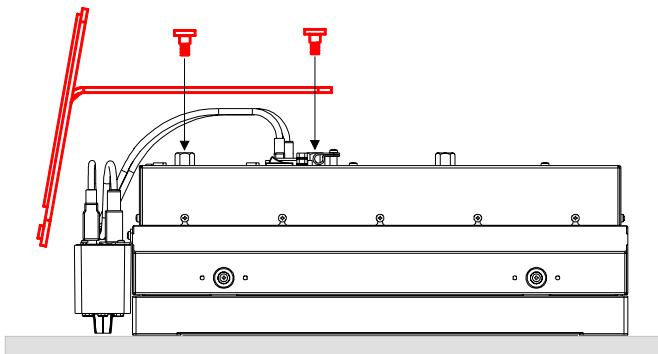
Figure 70: Mounting of Barco stand – screw location
