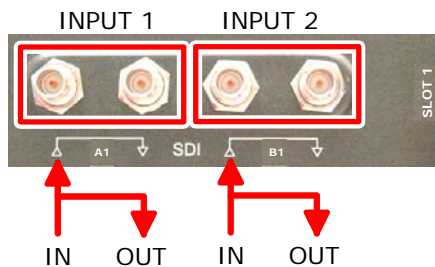
Figure 10: Input connectors SDI input board
