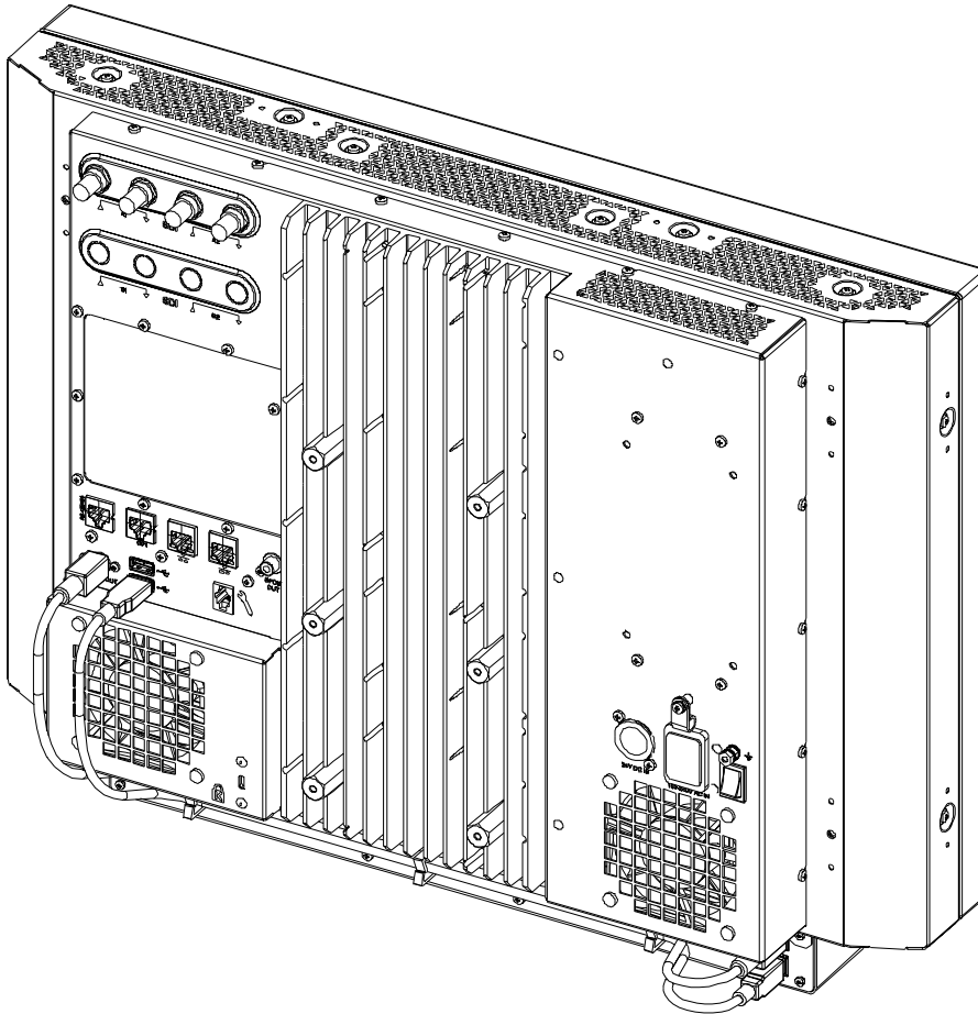
Figure 67: RHDM-2301 Auxiliary view (back)
