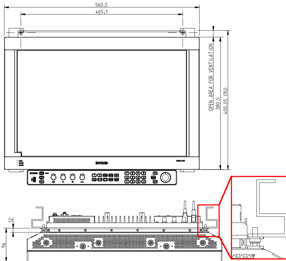
Figure 78: Installed display unit with control panel in an 19 inch rack
