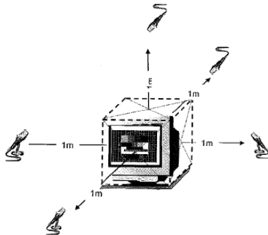
Figure 68: Setup to measure noise levels
