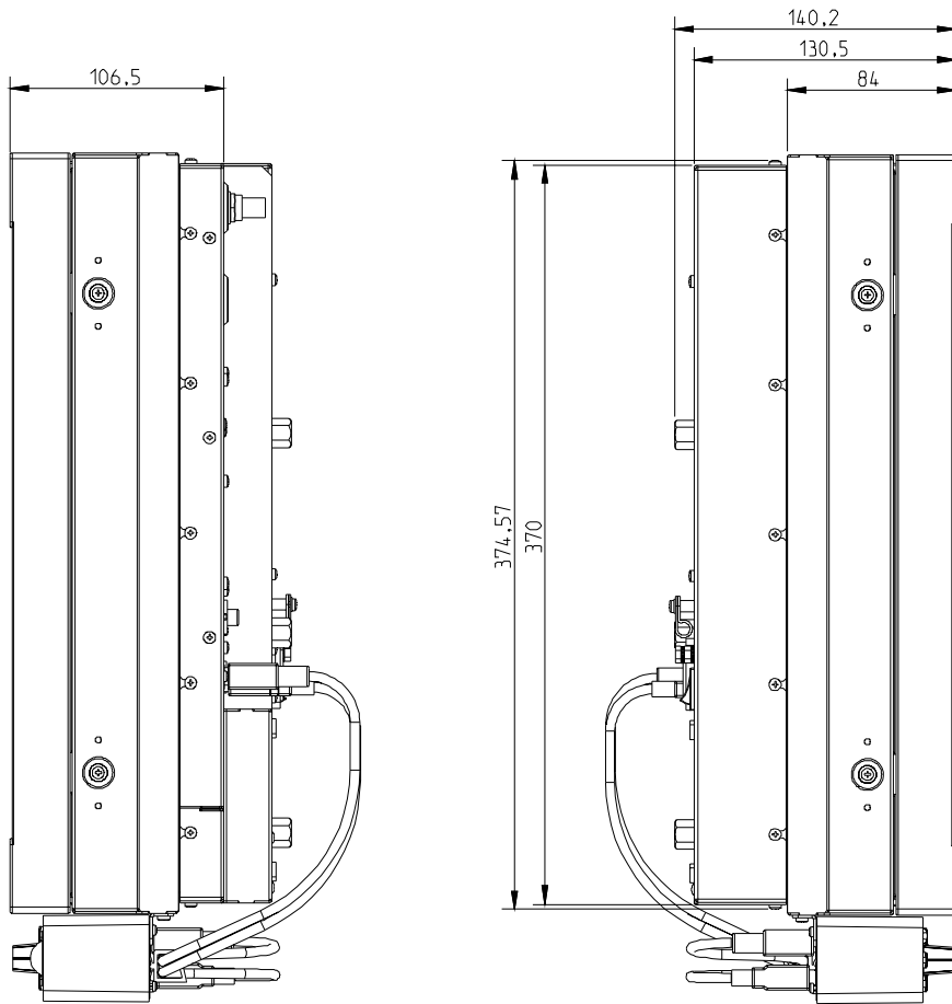
Figure 65: RHDM-2301 Side view (metric units (mm))
