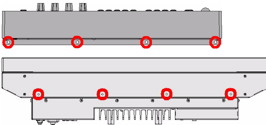
Figure 75: Bottom view of the control panel and the display unit
