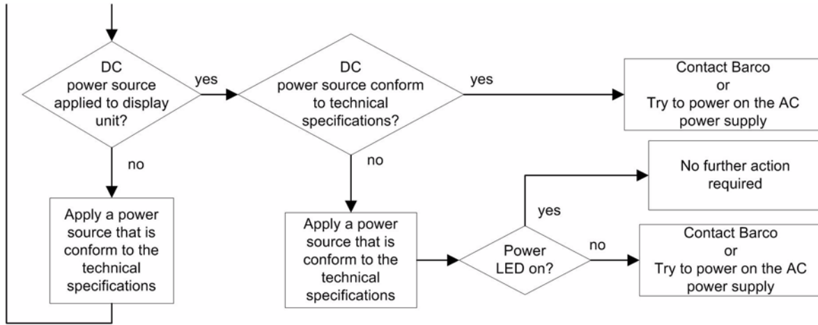
Figure 81: "No power" fault finding tree
