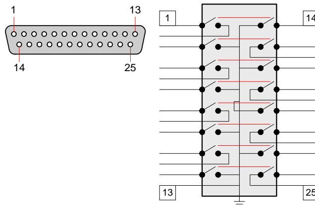
Figure A-6. Tally Connector and Circuit
