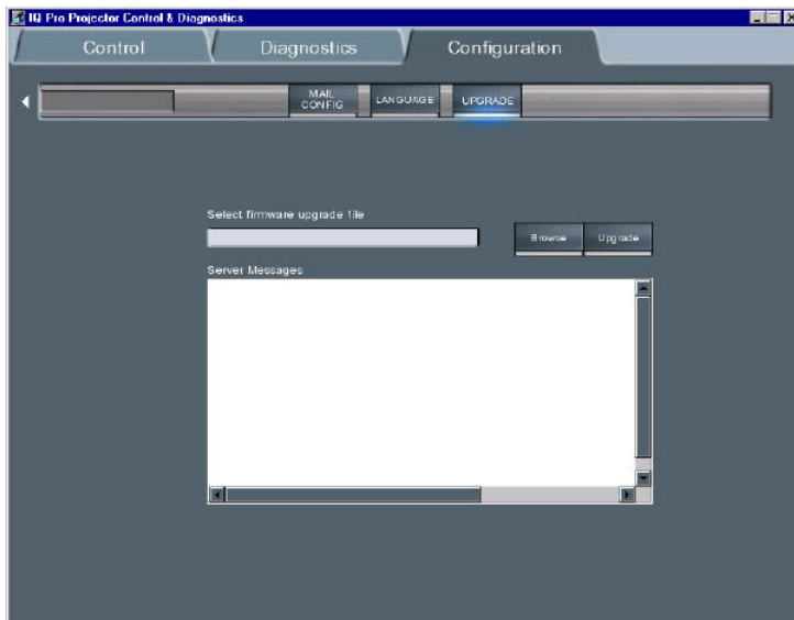
Image 9-28 upgrade interface
