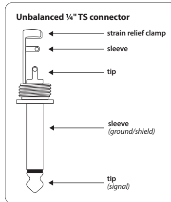
Fig. 7.1: ¼" TRS connector
