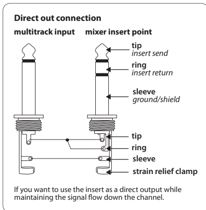
Fig. 7.5: Direct out connection
