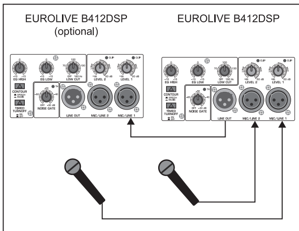
Fig. 4.1: Connecting microphones
