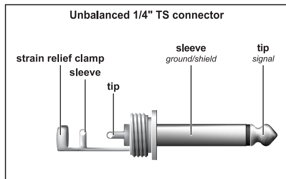
Fig. 4.1: 1/4" TS connector
