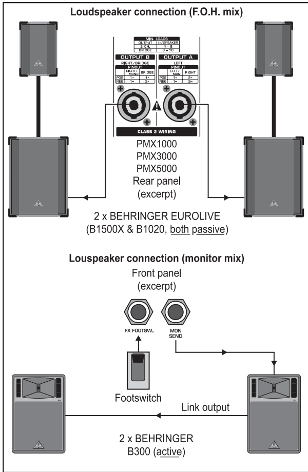
Fig. 5.1: Stereo operation
