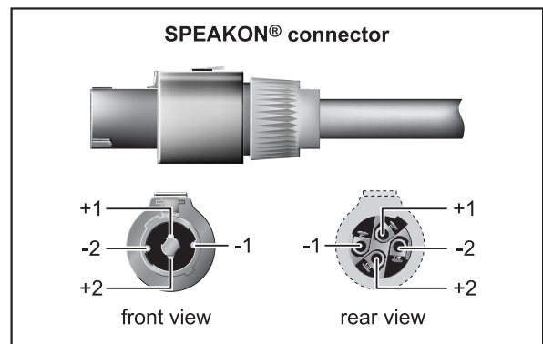
Fig. 4.5: SPEAKON® connector
