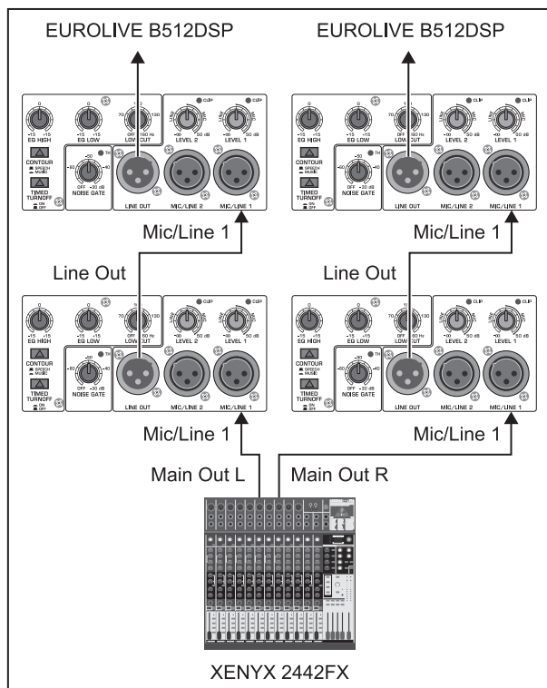
Fig. 4.3: Linking several B512DSP speakers
