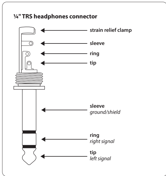
Fig. 7.2: ¼" TRS headphones connector
