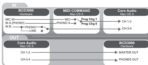
Fig. 5.6: Audio routing on the Mac
