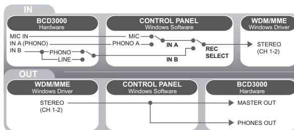
Fig. 5.5: Audio routing with the WDM/MME driver
