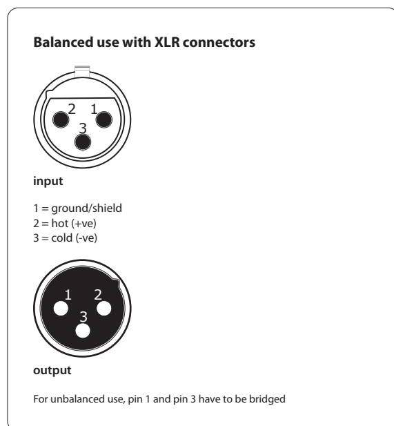
Fig. 7.1: XLR connector
