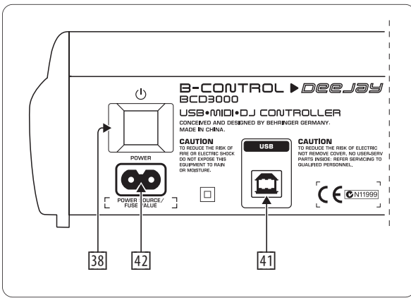
Fig. 3.3: POWER switch, mains and USB connectors
