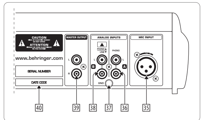
Fig. 3.2: The rear-panel audio connectors of the BCD3000
