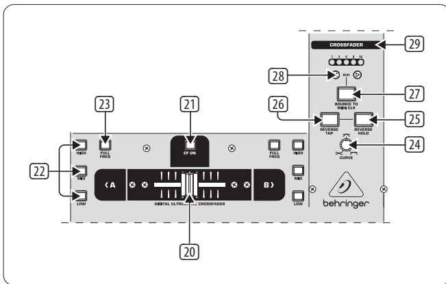
Fig. 2.3: Crossfader section
