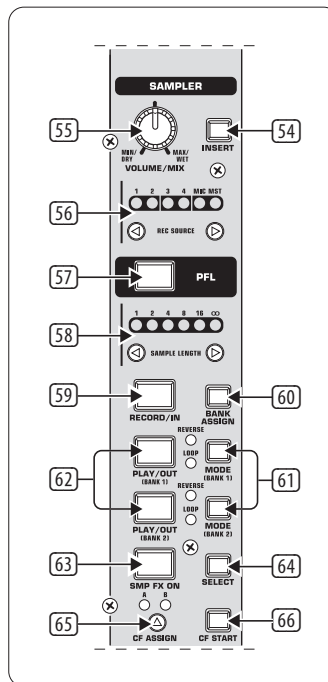
Fig. 5.1: Sampler section
