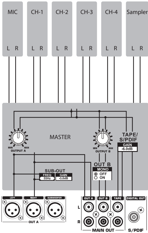
Fig. 10.2: Mixer routings
