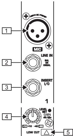
Fig. 2.1: Connectors and controls of the mic/line inputs
