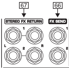
Fig. 2.26: FX send and return connectors
