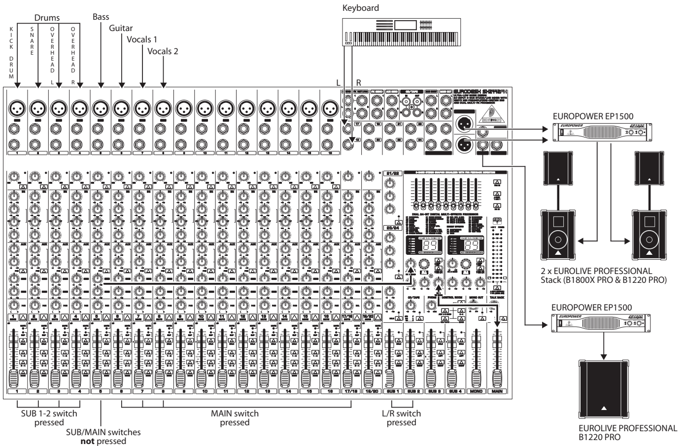
Fig. 4.2: Wiring the console for live operation
