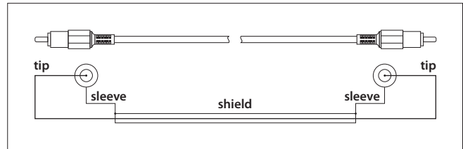
Fig. 5.3: RCA cable
