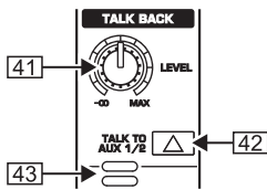
Fig. 2.17: Talkback section
