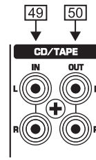
Fig. 2.21: CD/tape connectors
