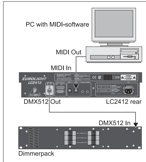
Fig. 7.4: MIDI connection
